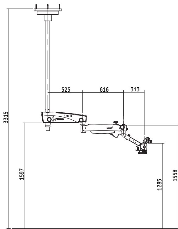
CEILING MOUNT
