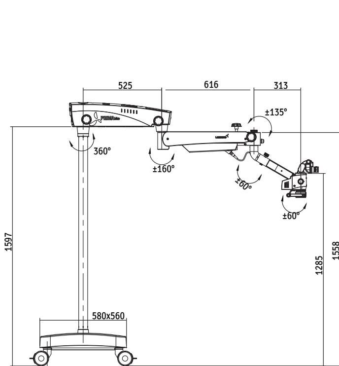
FLOOR MOUNT
